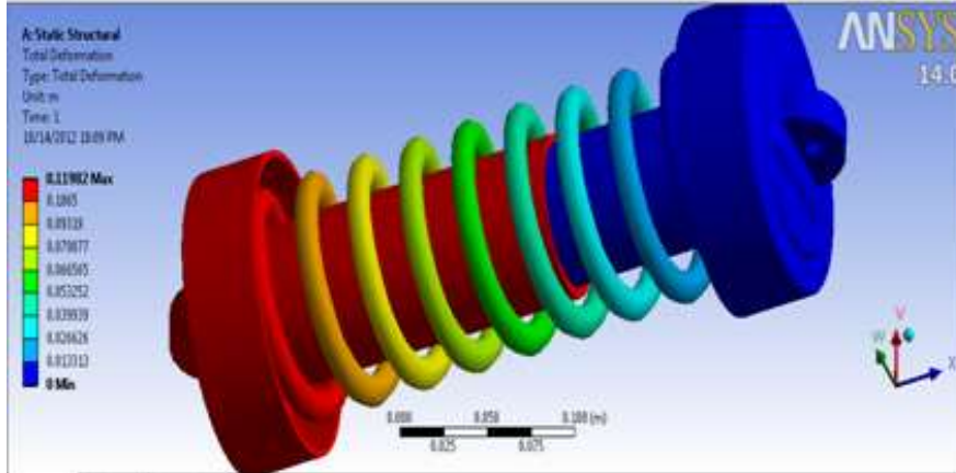
Fig. 6: Total deformation results
