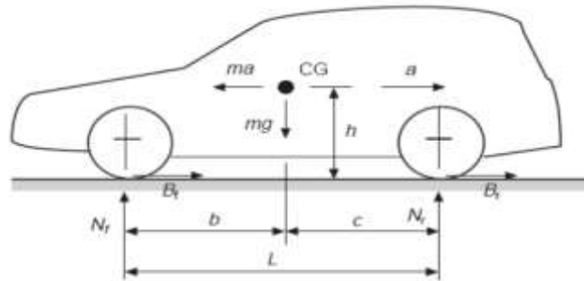
Fig. 2: Pitch analysis free body diagram Moment about the rear tyre gives -N_f L - mah - mgc = 0 -N_f = mah/L + mgc/L -N_f = mgb/L - mah/L ..... (11)
